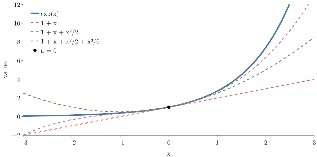
Figure 6: e^x and its Taylor approximations around 0: each extra term follows the curve over a wider range
