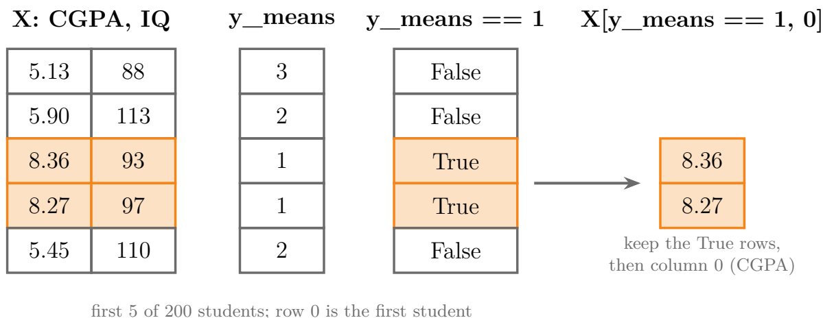
Figure 5: Boolean indexing on the first five students: the labels y_means , the mask y_means == 1 , and the CGPA values X[y_means == 1, 0] that the mask keeps
