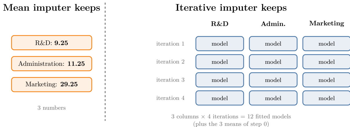
Figure 3: What each imputer keeps for production on the 5-row table: 3 means, against 12 fitted models for the default iterative imputer
