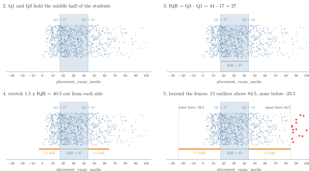
Figure 3: The IQR fences built step by step on the 1,000 exam marks: Q_1 and Q_3 , the IQR of 27, arms of 1.5 \text{ IQR} , then the 15 outliers beyond 84.5
