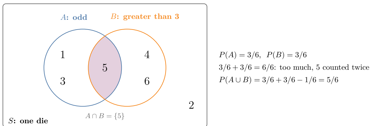
Figure 3: The general addition rule on one die: the overlap \{5\} is counted twice by P(A) + P(B)
