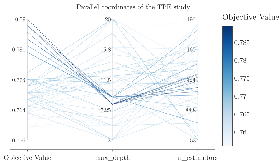
Figure 4: Parallel coordinates of the TPE study: each line is a trial, darker is a higher score
