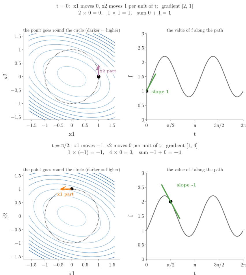
Figure 10: A point goes round the unit circle on the contour map of the bowl (left); the right panel tracks the value of f . At t = 0 the step is all along x_2 (purple) and f rises with slope 1; at t = \pi/2 it is all along x_1 (orange) and f falls with slope -1 . Idea after Khan Academy, “Multivariable chain rule” and “Multivariable chain rule intuition”; our own function
