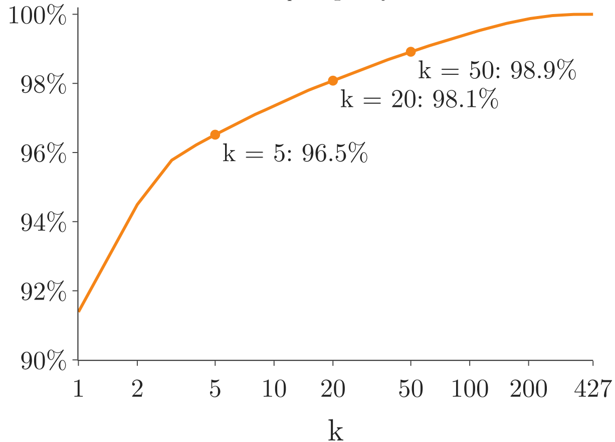
share of \sum \sigma_i^2 kept by the first k
