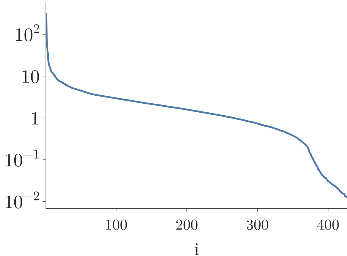
singular values \sigma_i (log scale)
