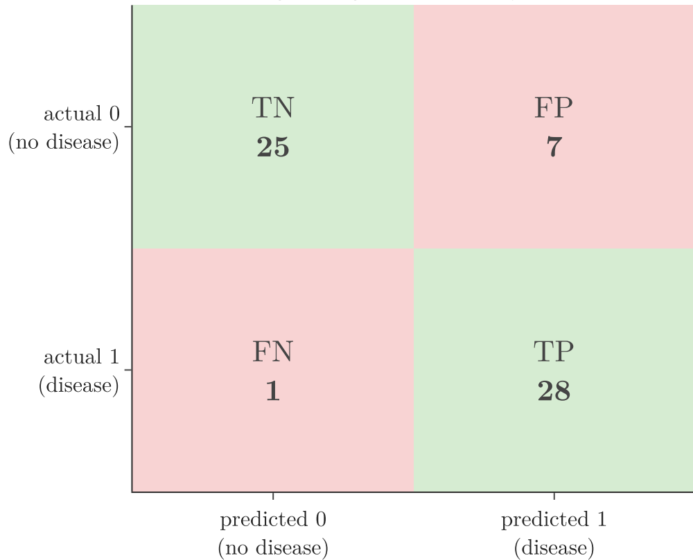
Logistic regression: accuracy 0.869
