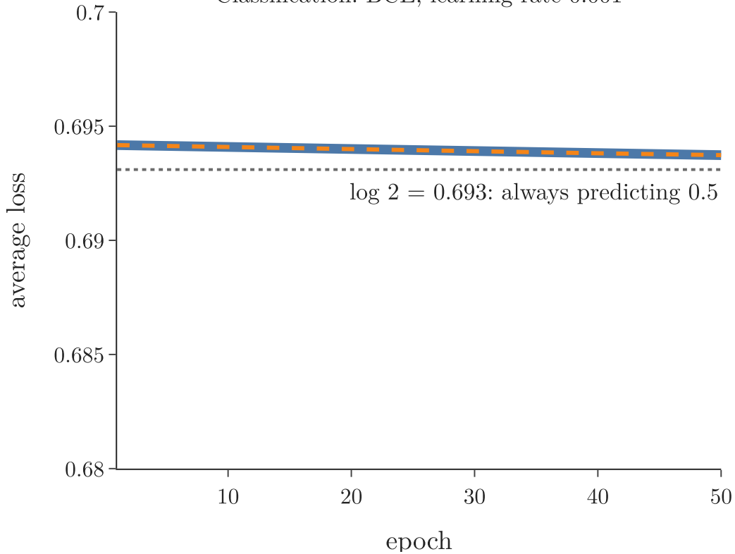
Classification: BCE, learning rate 0.001
