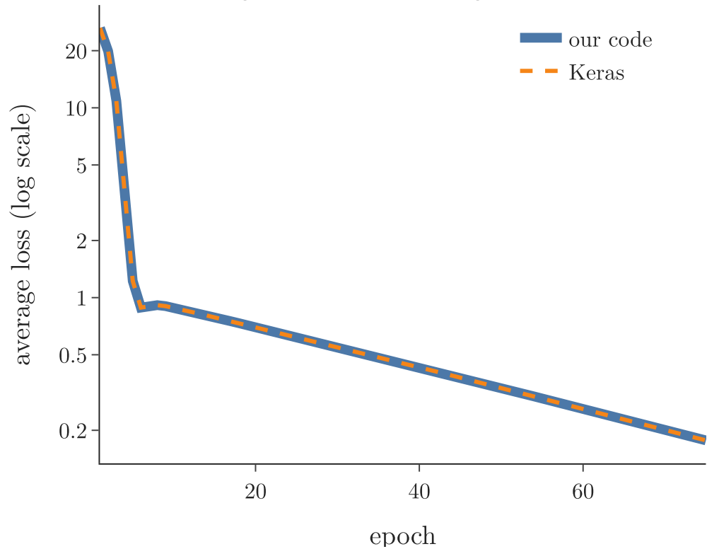
Regression: MSE, learning rate 0.001
