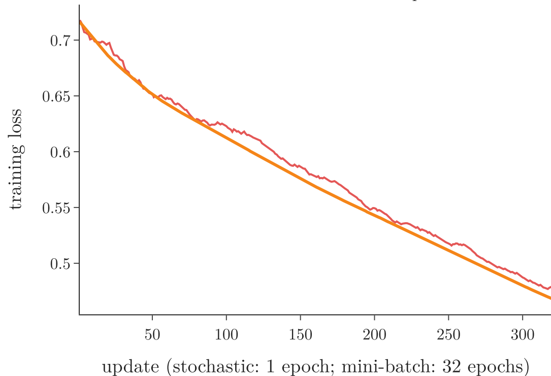
Loss after each of the first 320 updates
