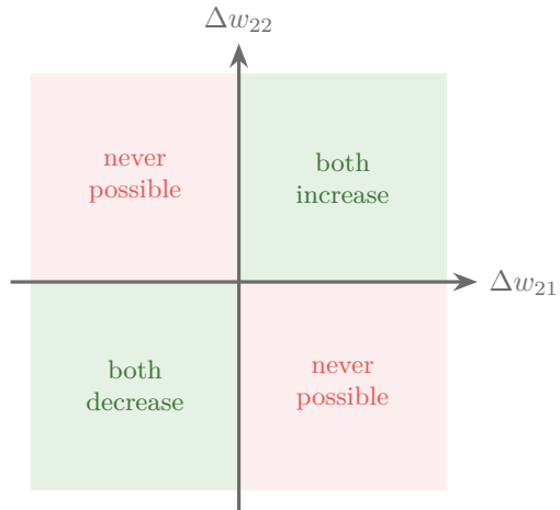
(a) Directions one update can take
