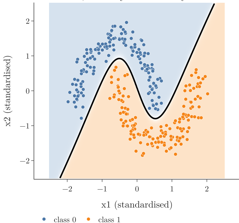
tanh, Xavier by hand: accuracy 100%
