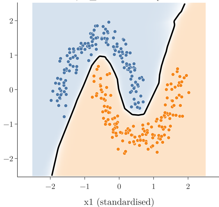
ReLU, he_normal: accuracy 100%
