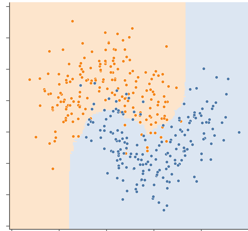
pasting 50 rows, without replacement: 0.904
