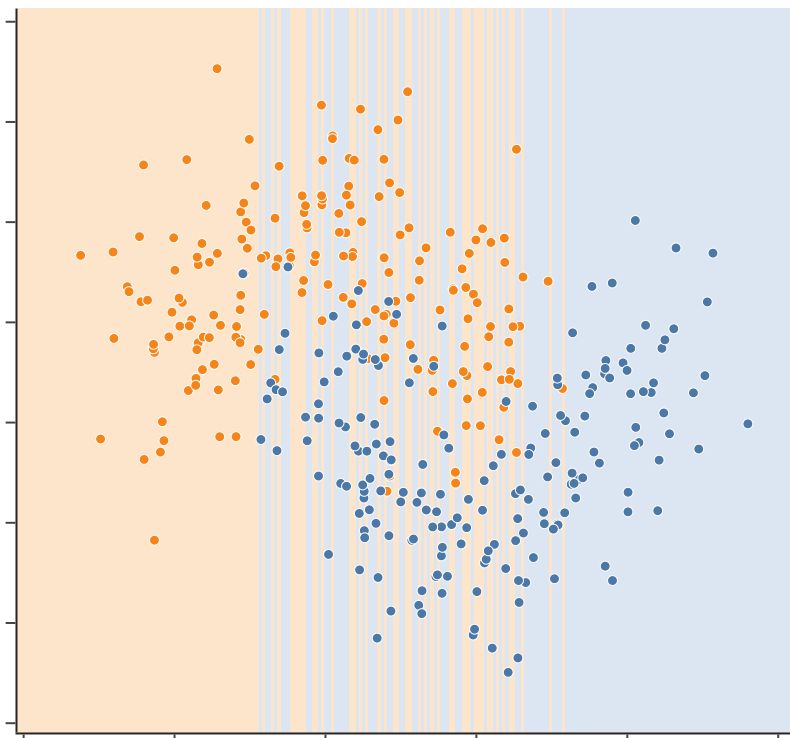
random subspaces all rows, 1 of 2 columns: 0.648
