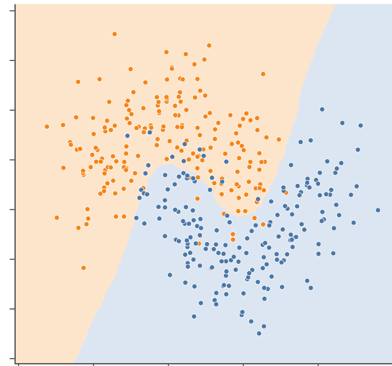
bagged KNN 50 rows, with replacement: 0.912
