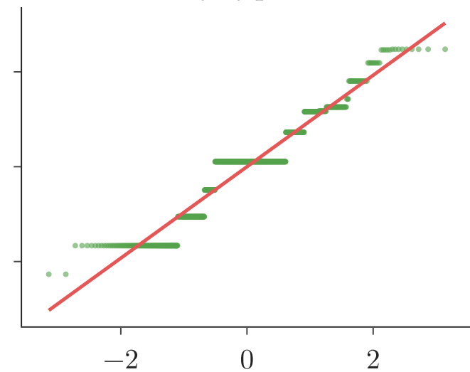
Q-Q plot
