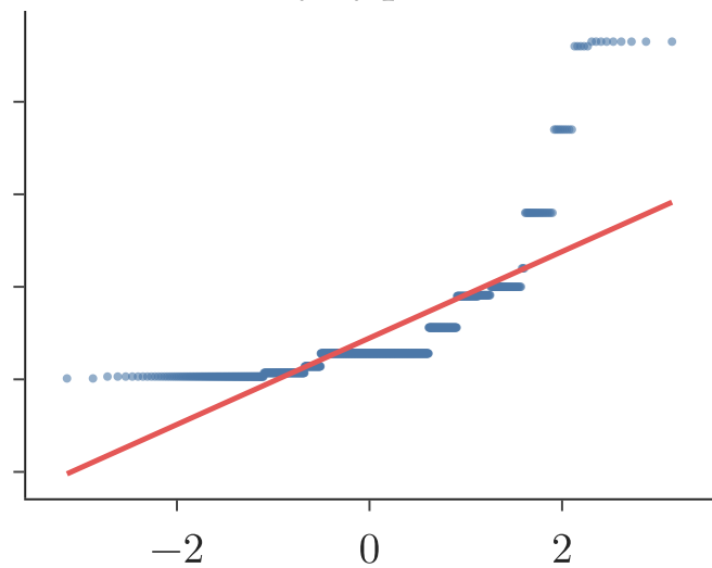
Q-Q plot
