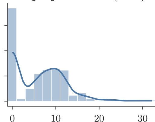
Superplasticizer (0.90)
