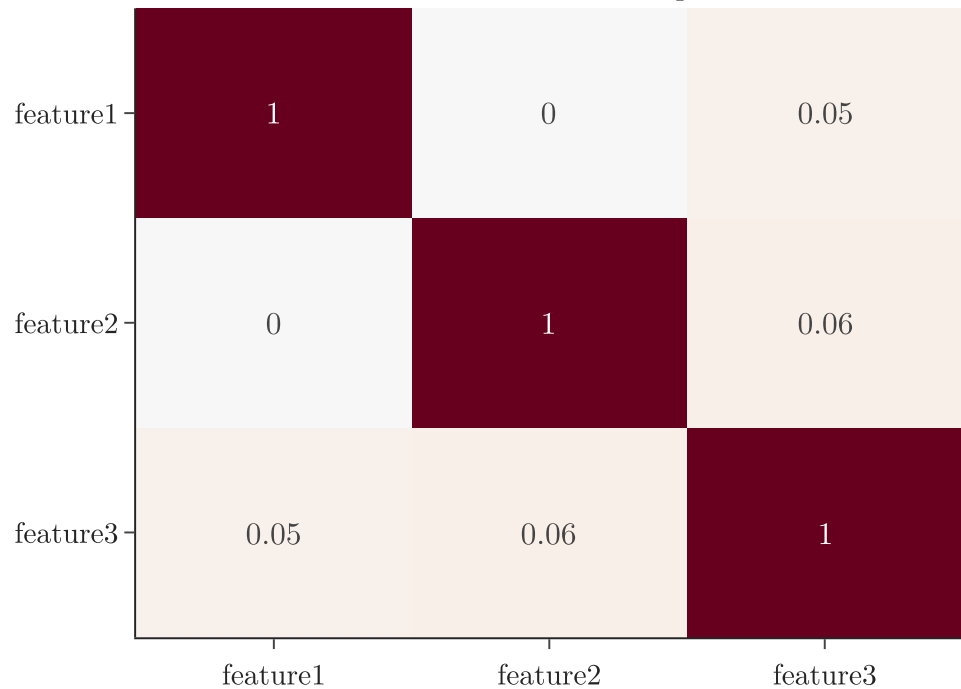
Correlation between inputs
