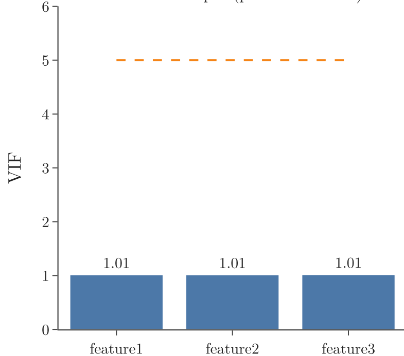
VIF of each input (problem above 5)
