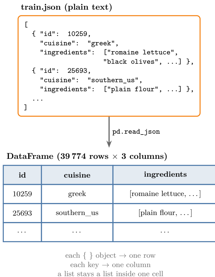
Figure 2: From JSON text to a DataFrame
