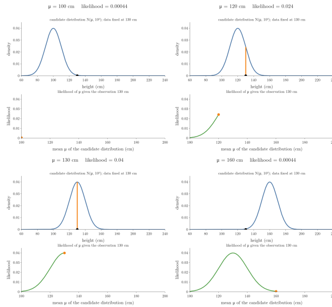
Figure 3: One person measured at 130 cm. Top: the candidate curve N(\mu, 10^2) slides; the orange bar is its height at 130. Bottom: those heights against \mu , the likelihood function, highest at \mu = 130
