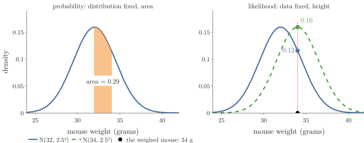
Figure 4: Mouse weights. Left: probability as the area between 32 and 34 grams under N(32, 2.5^2) . Right: likelihood as the height at the observed 34 grams, for two candidate distributions
