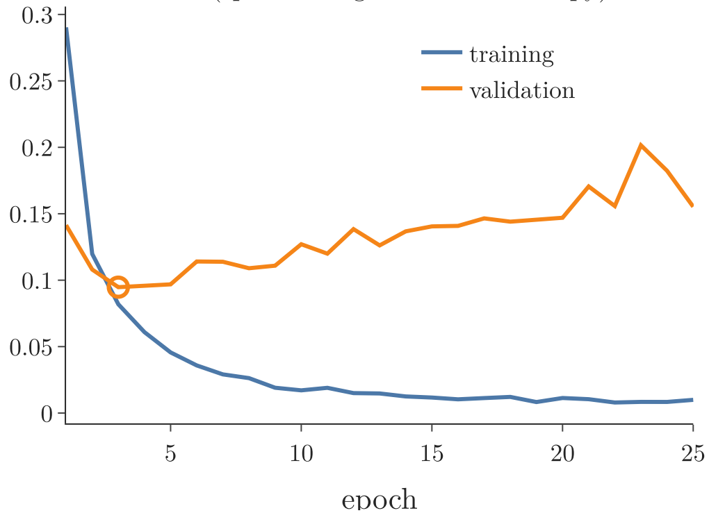
Loss (sparse categorical cross-entropy)
