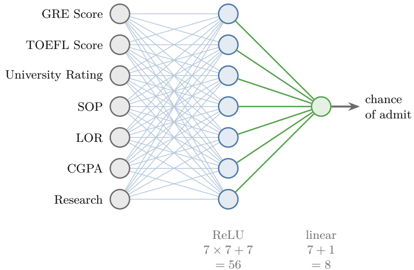
(a) First network: 7-7-1
