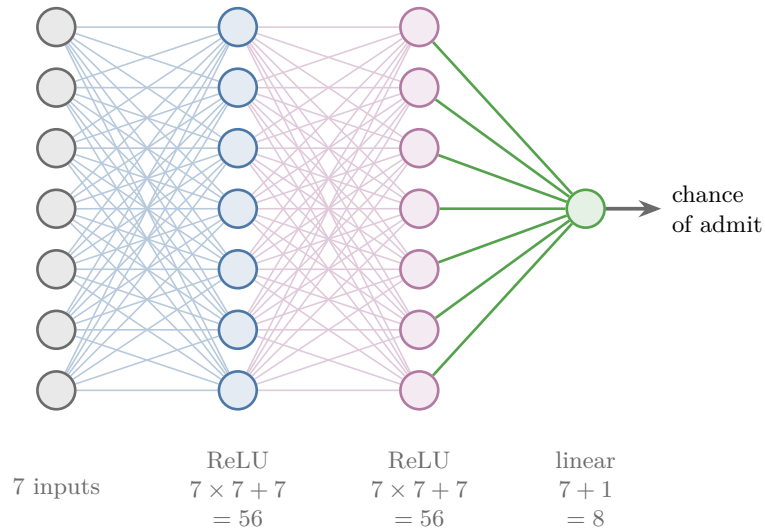
(b) Second network: 7-7-7-1
