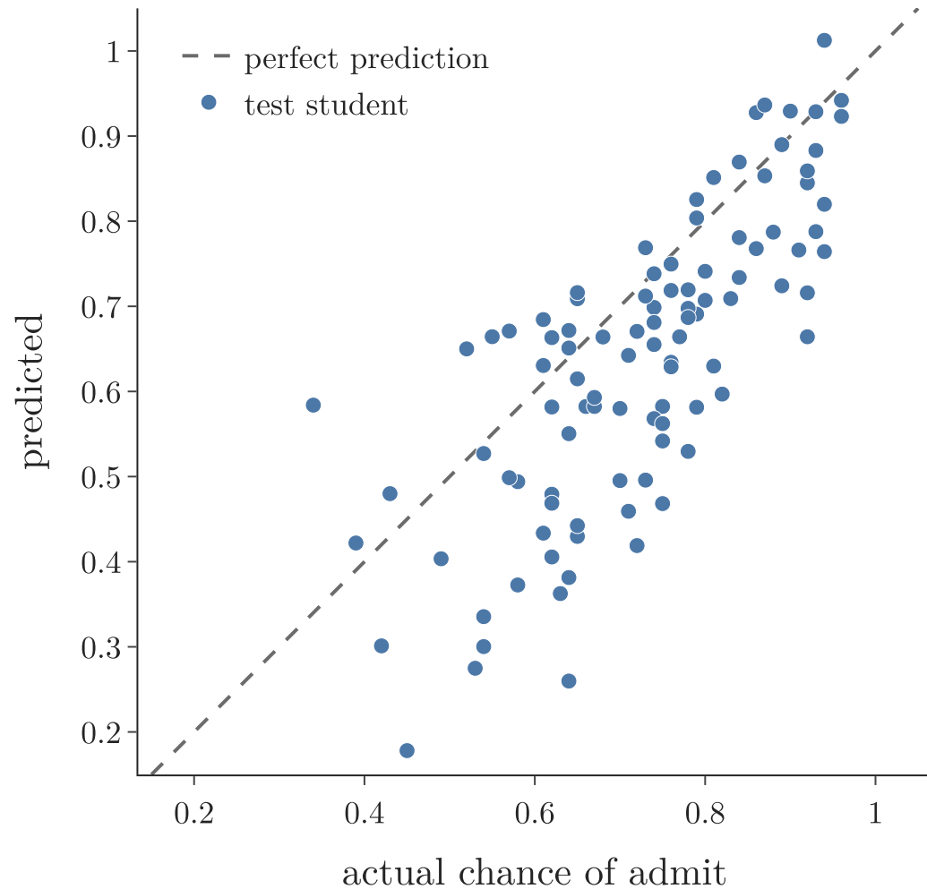
First network: R^2 = -0.06
