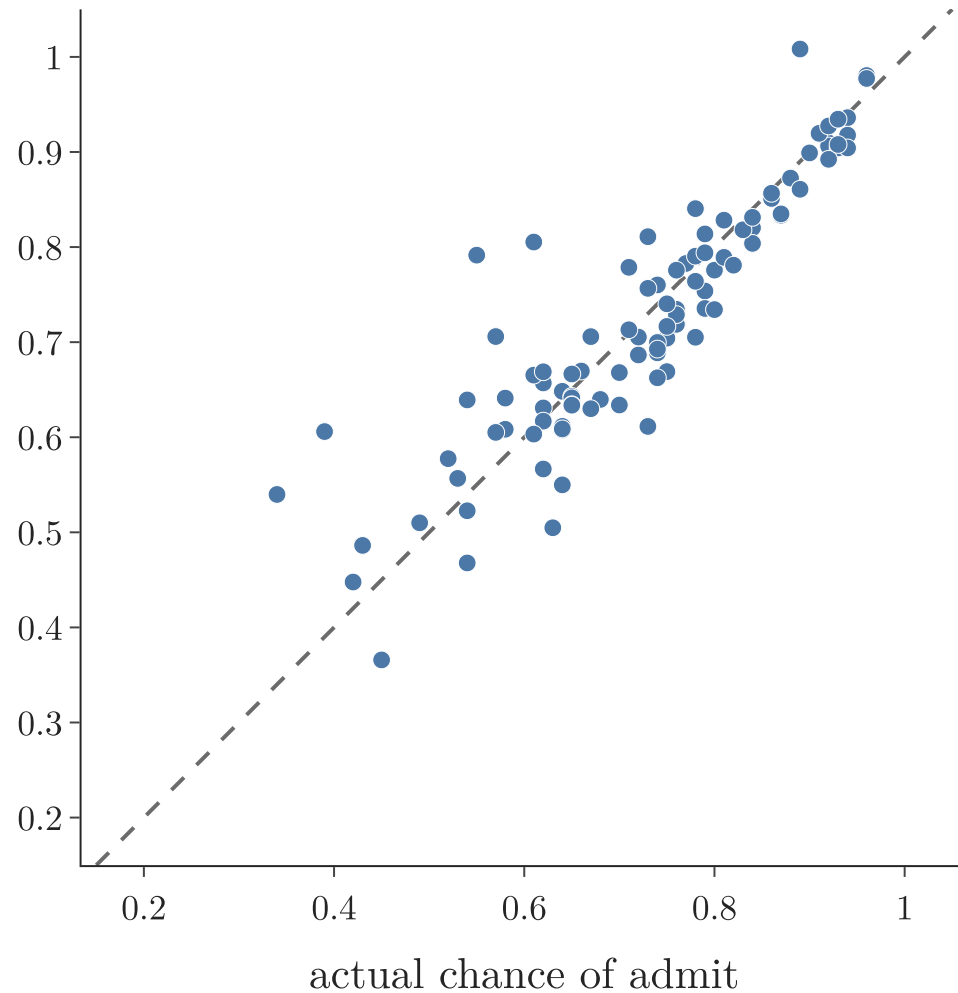
Second network: R^2 = 0.80
