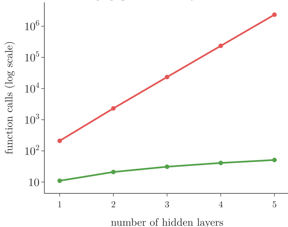
Backpropagation: hidden layers of 10 nodes
