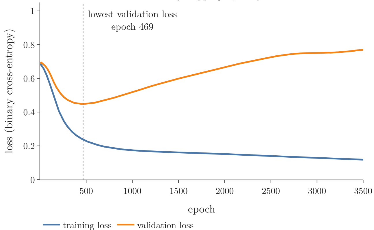
Without early stopping: 3,500 epochs
