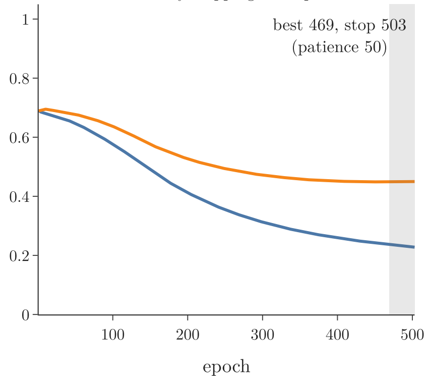
With early stopping: 503 epochs
