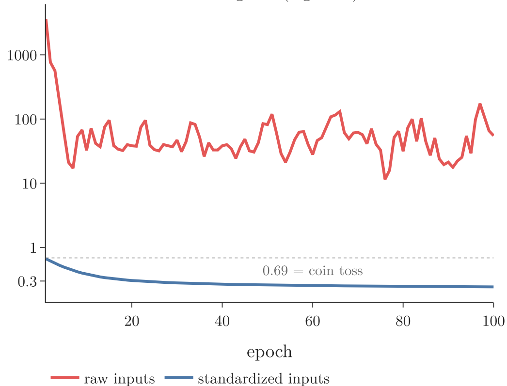
Training loss (log scale)
