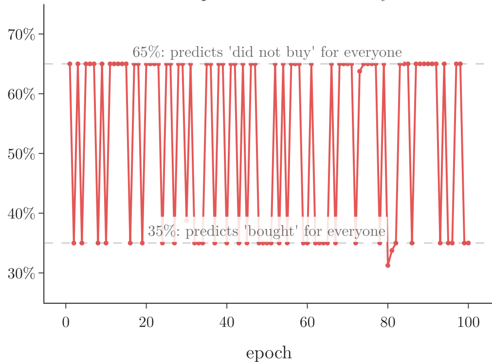
Raw inputs: validation accuracy
