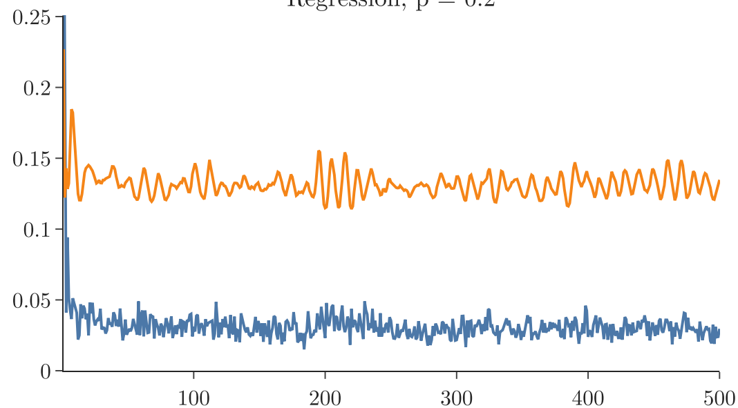
Regression, p = 0.2
