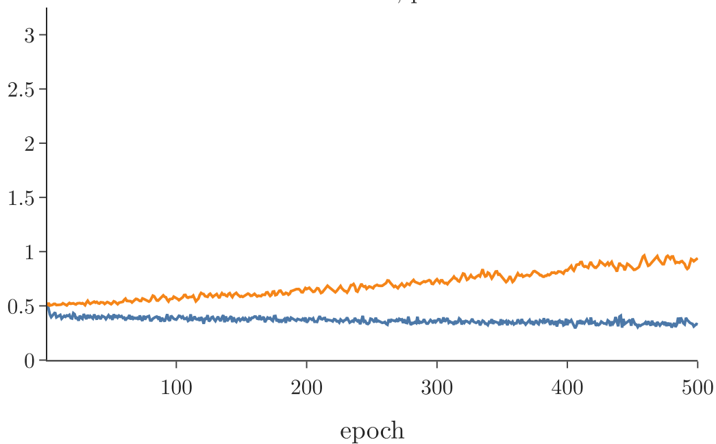
Classification, p = 0.5
