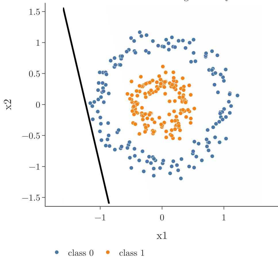
Linear activation: training accuracy 50%
