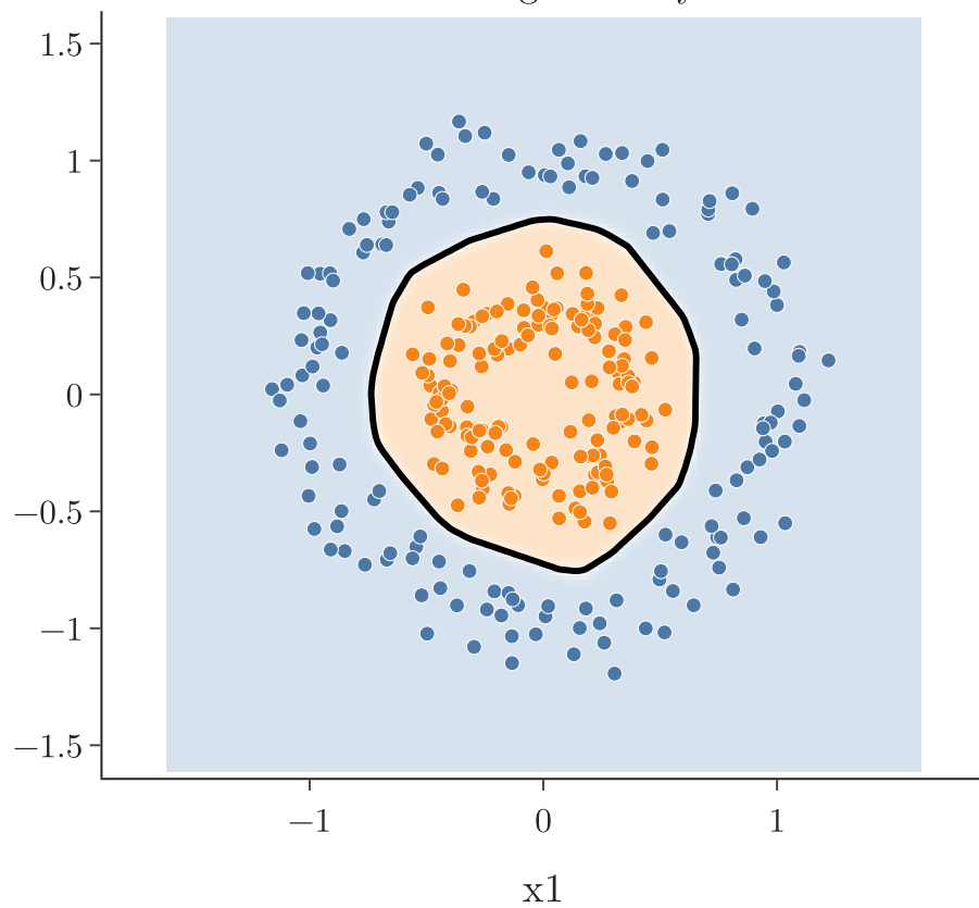
ReLU: training accuracy 100%
