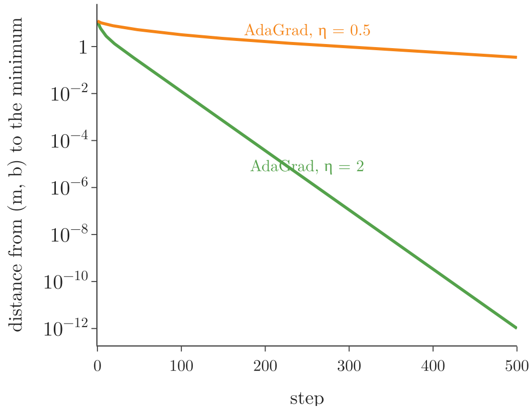
distance to the minimum
