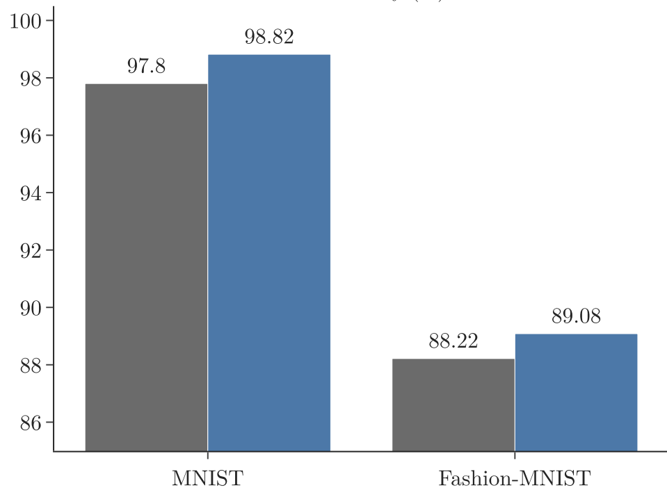
test accuracy (%)
