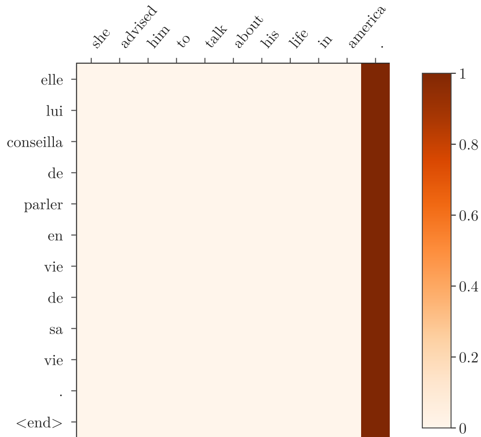
Luong general
