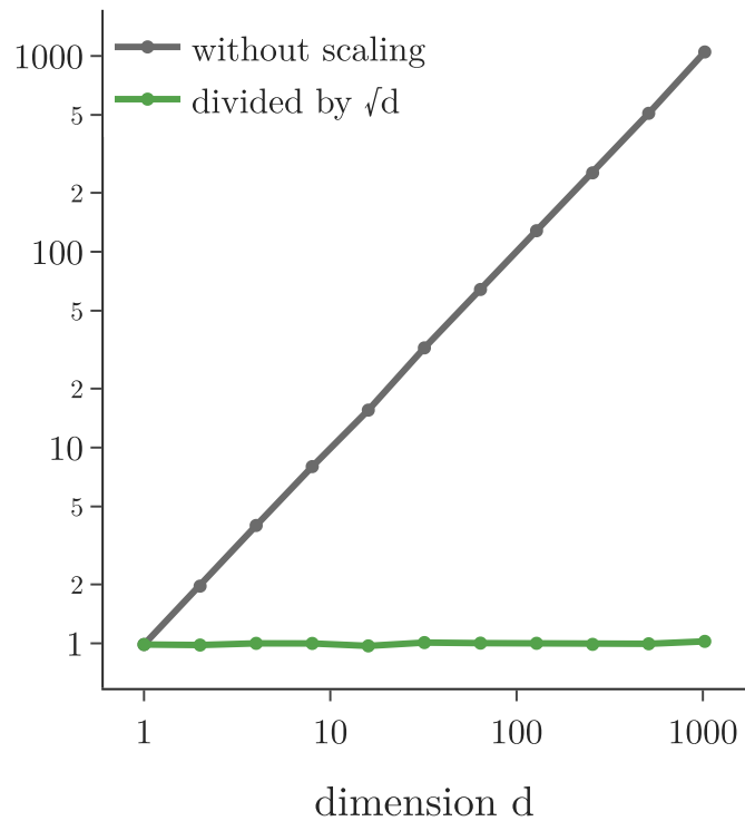
variance of the scores
