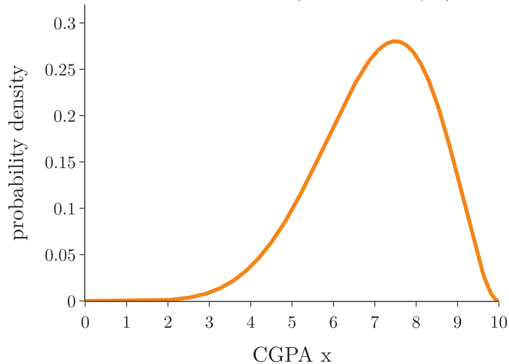
Continuous: CGPA (a value at every x)
