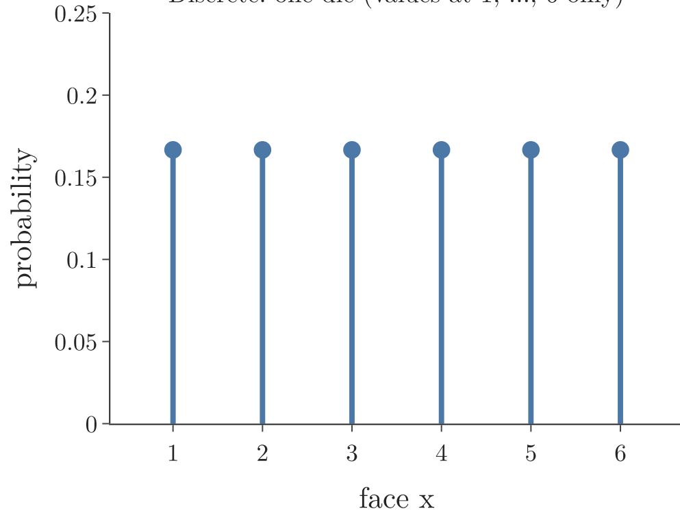
Discrete: one die (values at 1, ..., 6 only)
