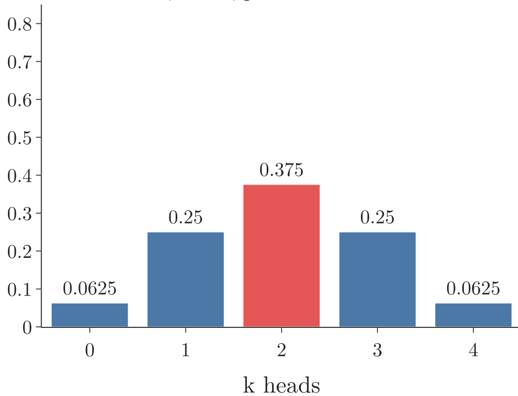
binomial, n = 4 , p = 0.5 : heads in 4 tosses
