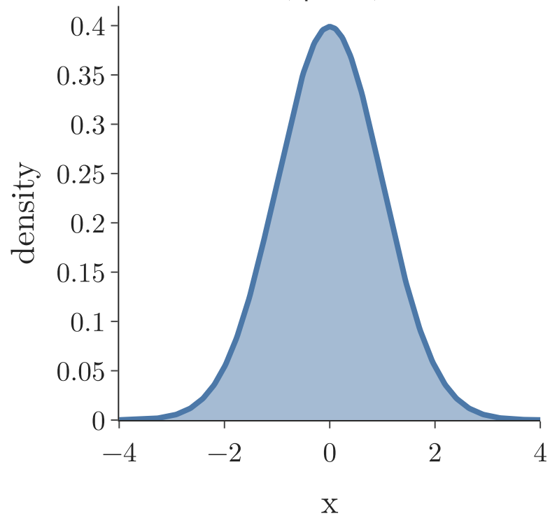
normal, \mu = 0, \sigma = 1
