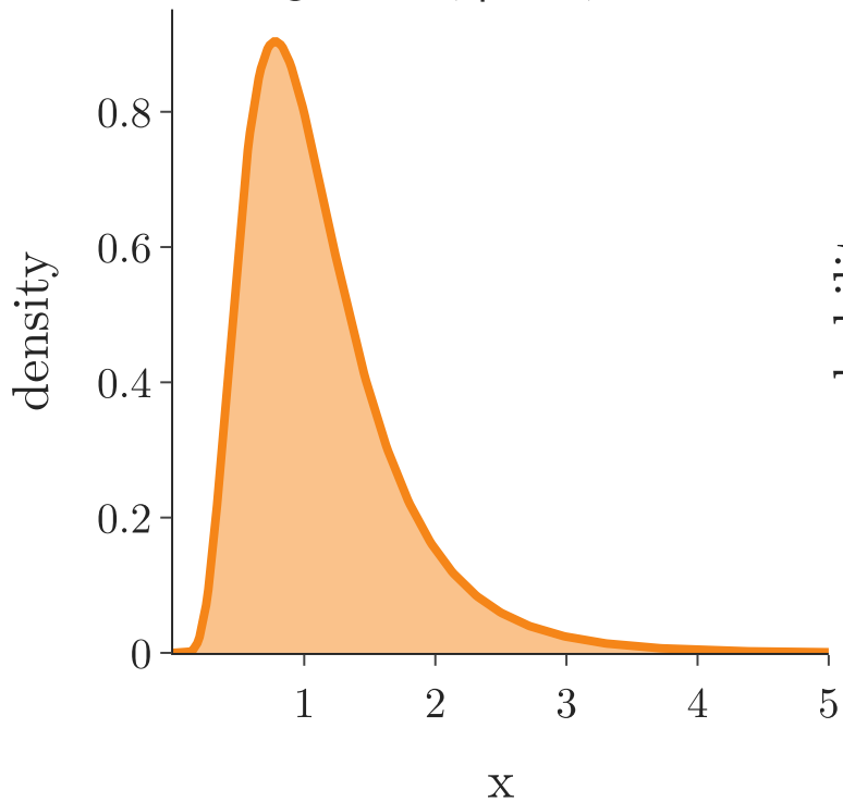
log-normal, \mu = 0, \sigma = 0.5
