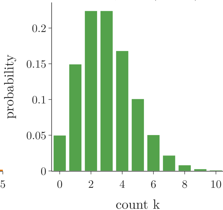
Poisson, \lambda = 3 (discrete)
