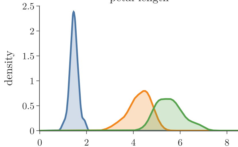
petal length
