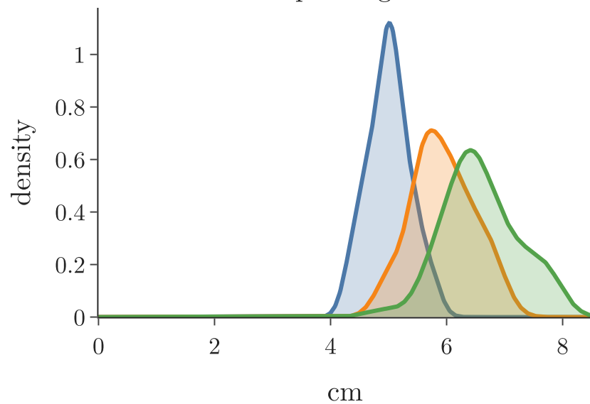
sepal length
