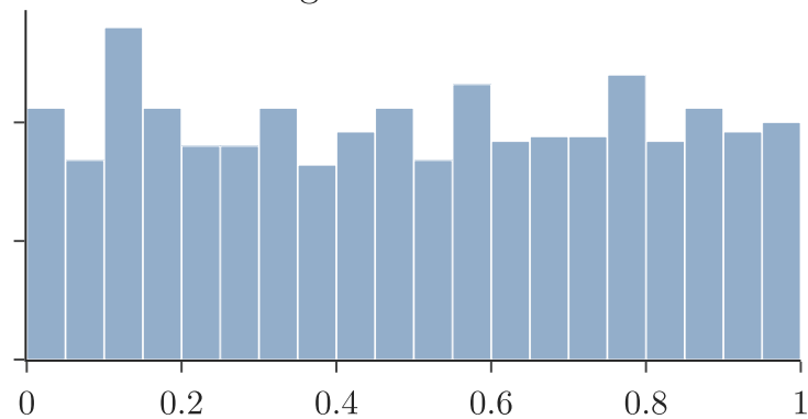
Same uniform data against uniform
