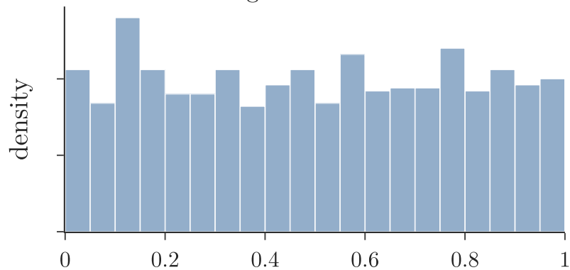
Uniform, thin tails (excess kurtosis -1.2) against normal
