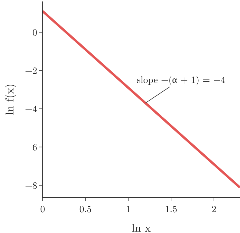
PDF formula, log-log axes
