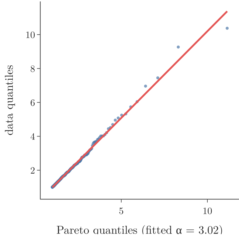
Q-Q plot against Pareto
