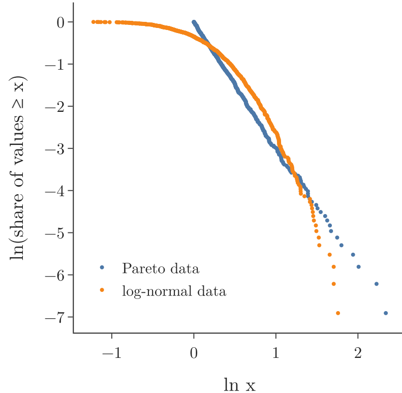
Data: share above x, log-log axes
