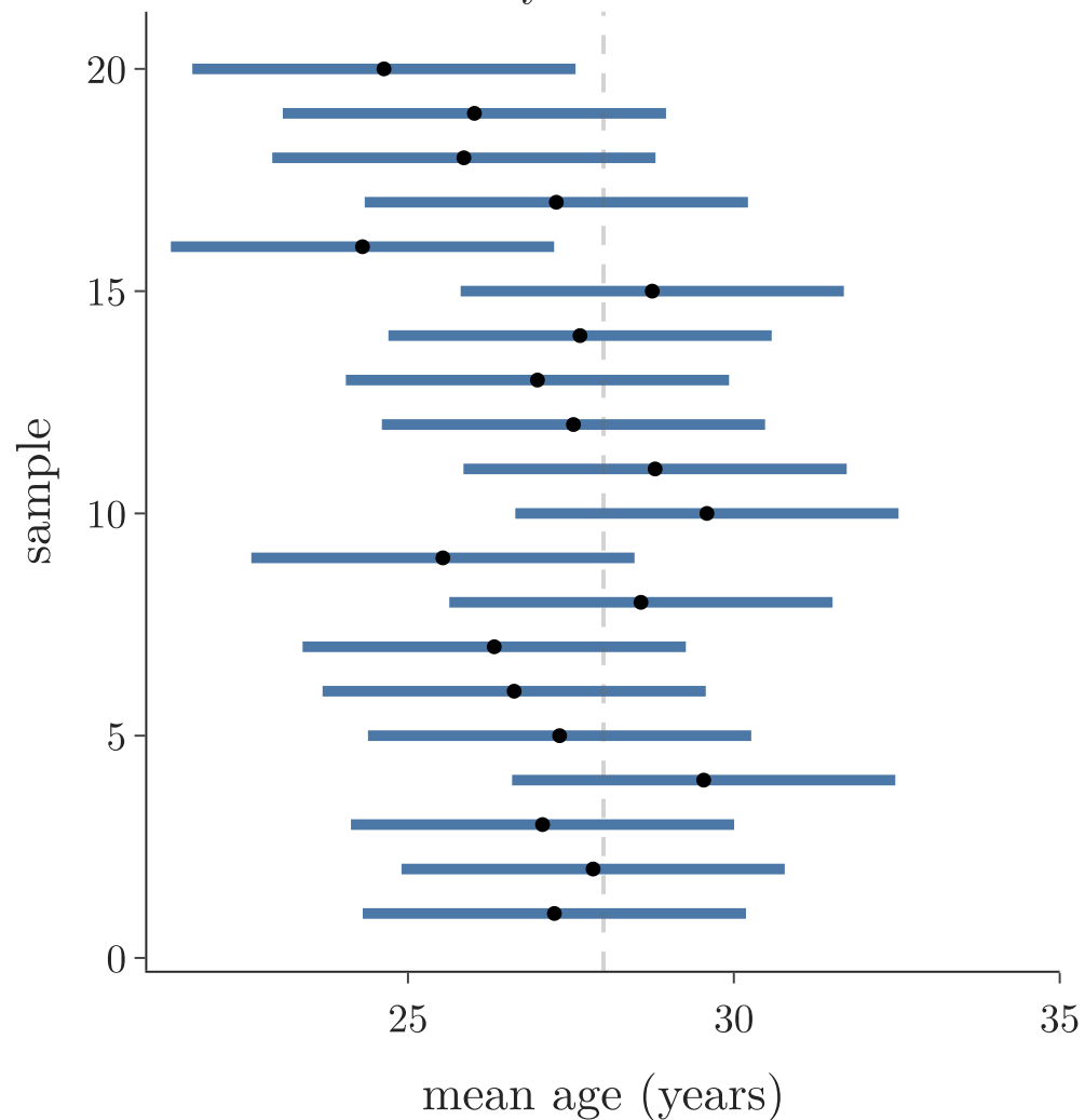
z-procedure: \sigma = 15 known every width 5.88
