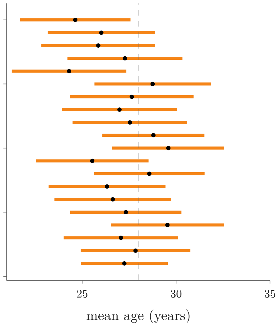
t-procedure: s from each sample widths 4.62 to 6.58
