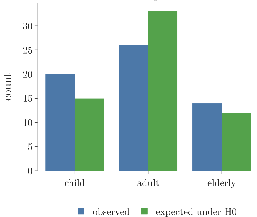
observed and expected counts
