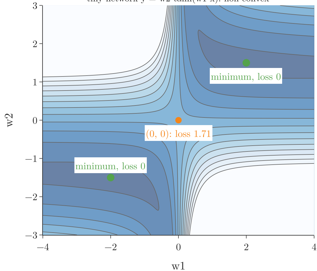
tiny network y = w_2 \tanh(w_1 x) : non-convex
