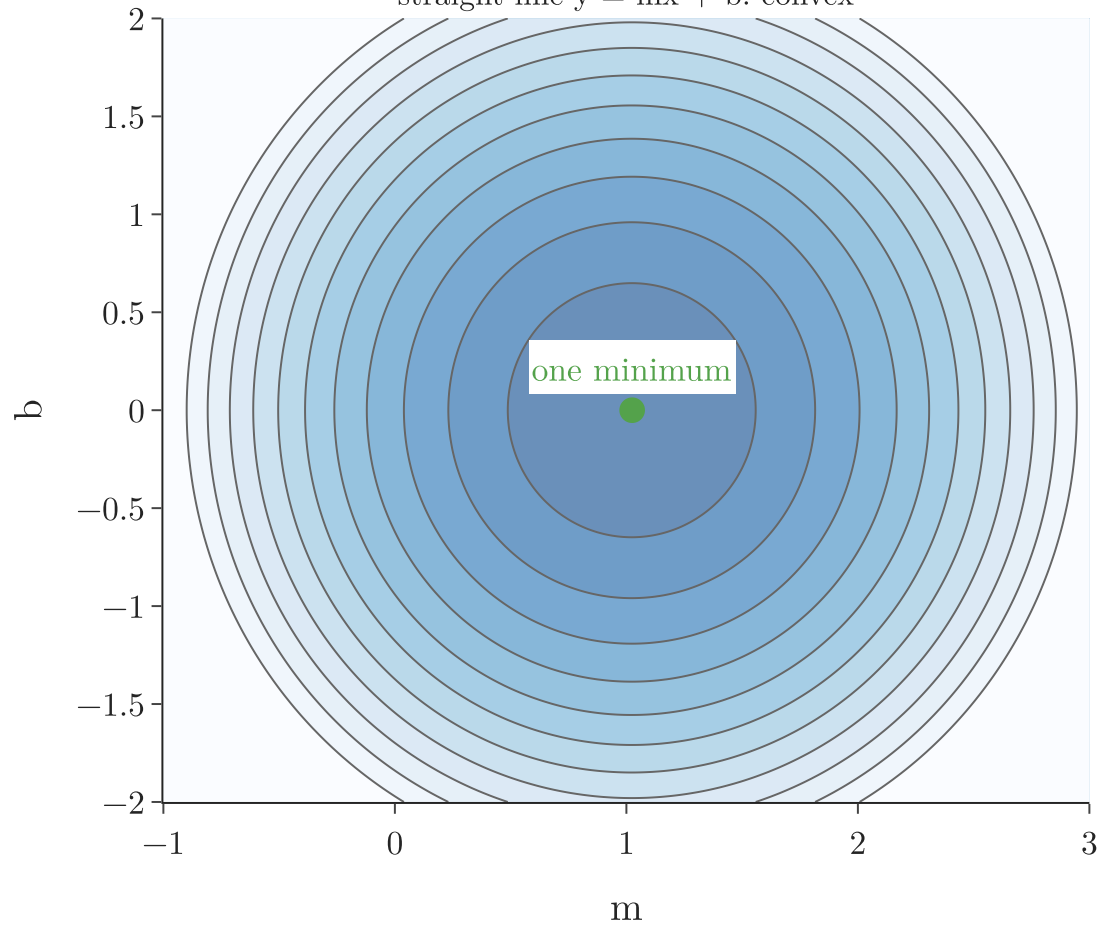
straight line y = mx + b : convex
