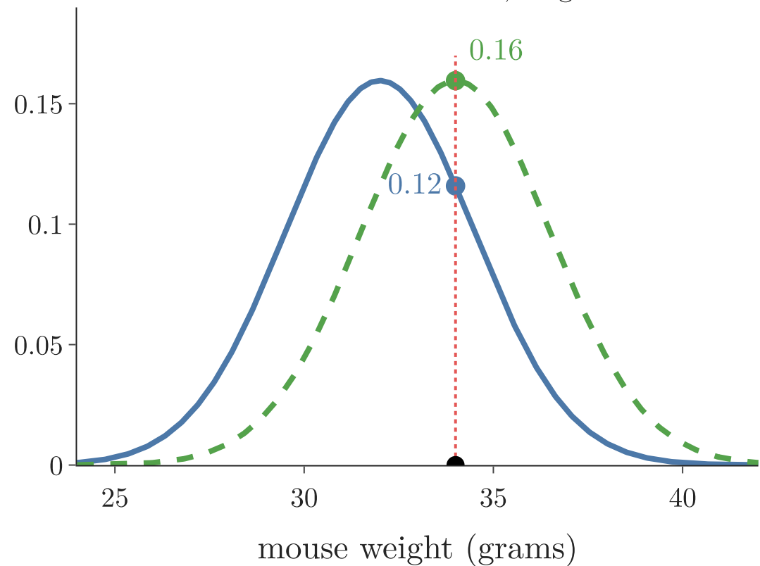
likelihood: data fixed, height
