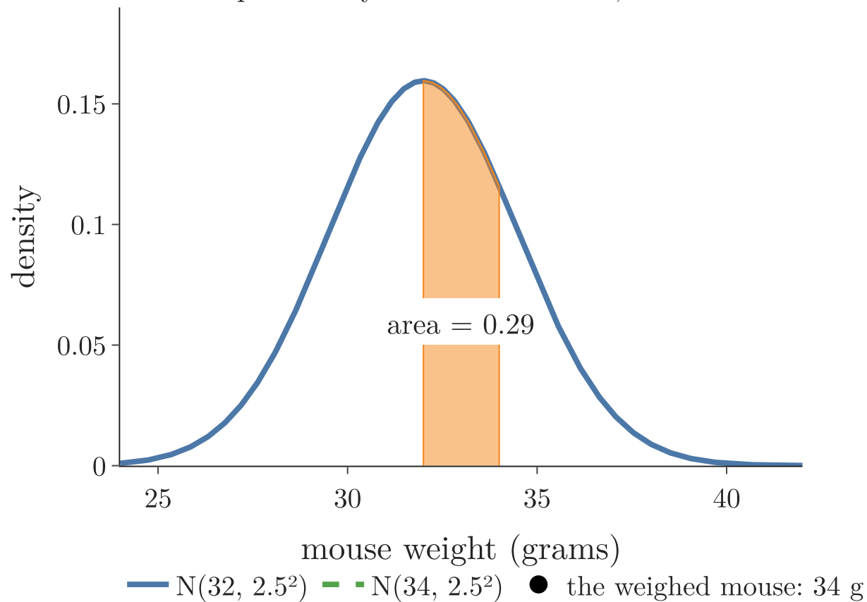
probability: distribution fixed, area
