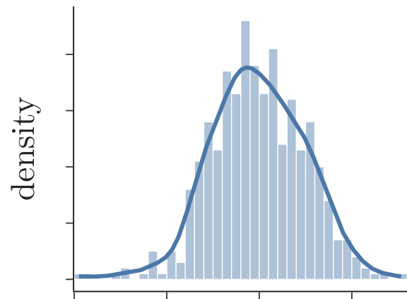
Normal
