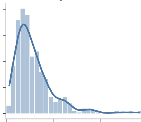
Right skew
