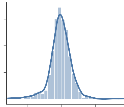
Fat tails
