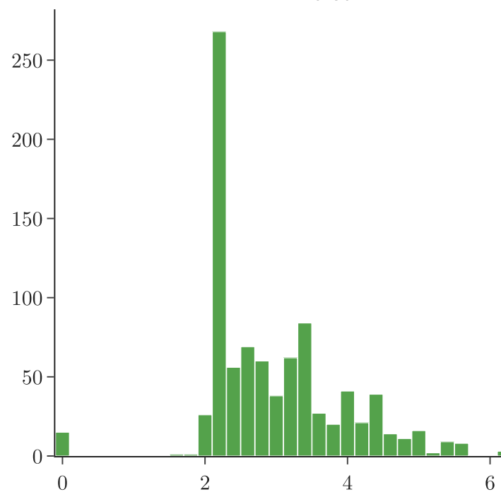
FunctionTransformer(np.log1p) skewness 0.39
