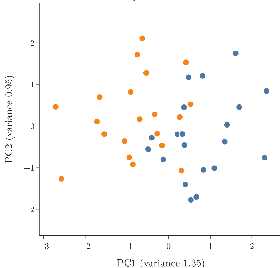
The same points on PC1 and PC2
