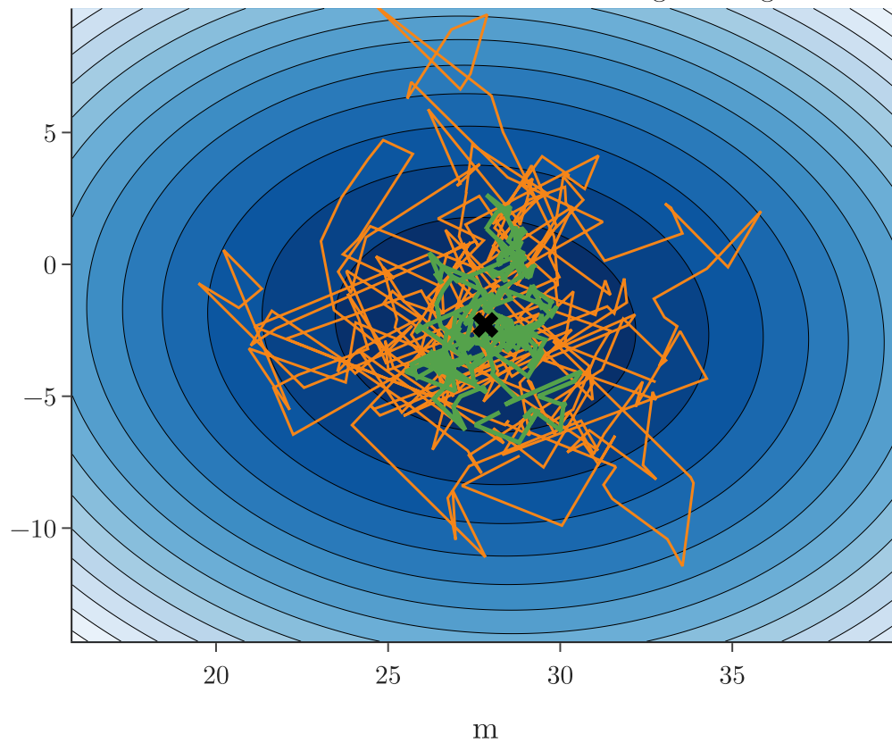
Near the minimum: constant vs decreasing learning rate
