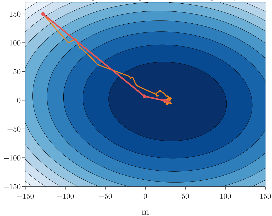
10 batch updates vs 1 epoch of SGD (100 updates)
