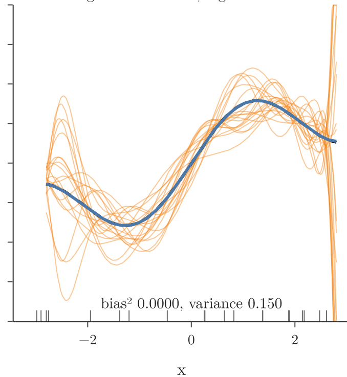
Degree 11: low bias, high variance
