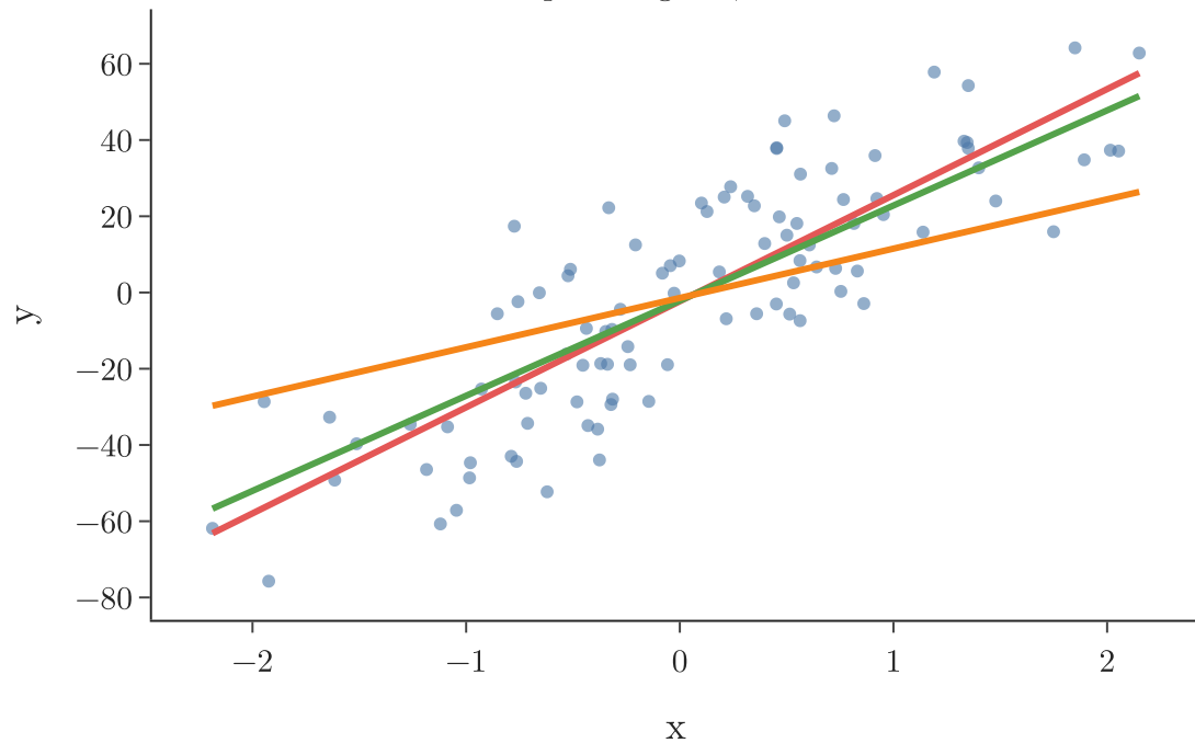
One input: larger \alpha , flatter line
