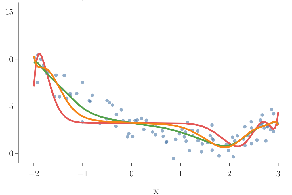
Degree 16: \alpha = 0 overfits, \alpha = 200 underfits
