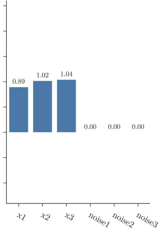
Elastic Net (alpha 0.1, l1_ratio 0.5)
