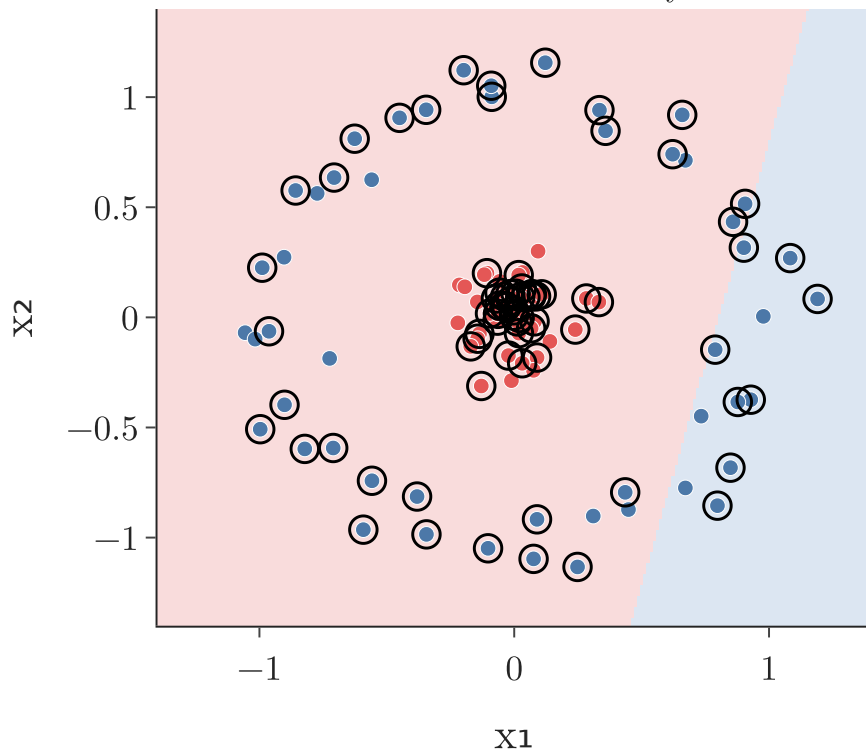
linear kernel: test accuracy 0.55
