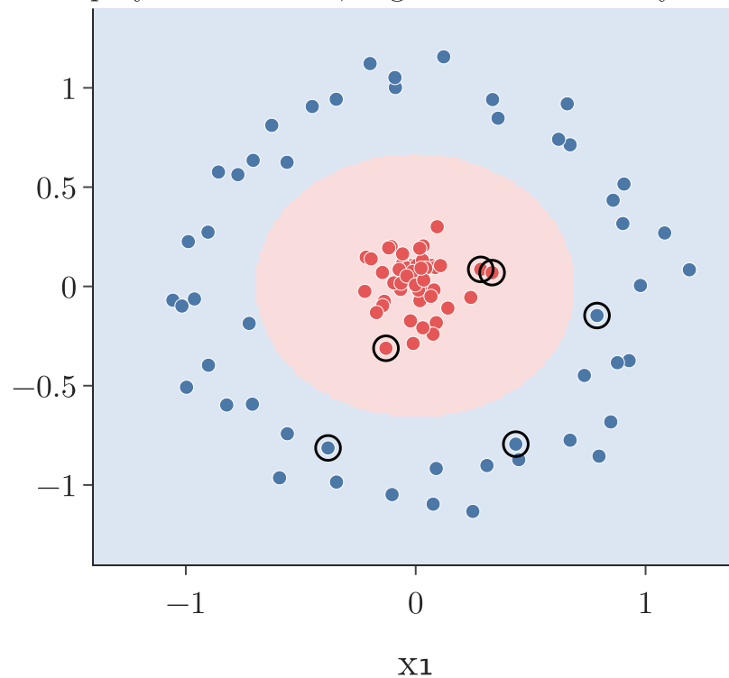
polynomial kernel, degree 2: test accuracy 1.00
