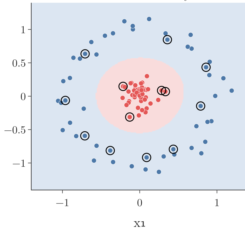
RBF kernel: test accuracy 1.00
