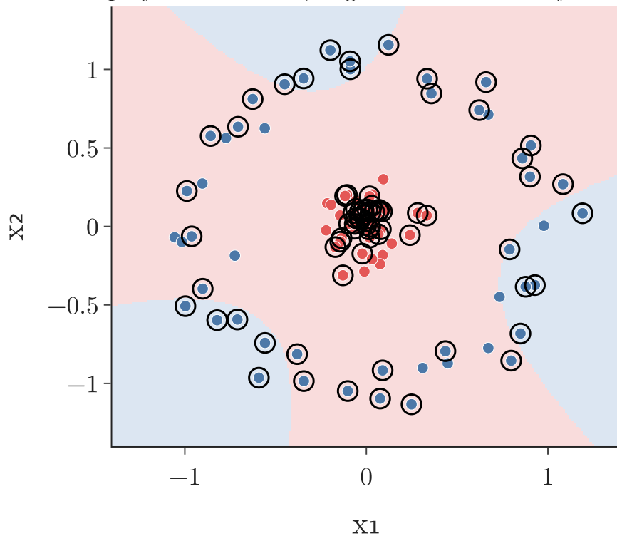
polynomial kernel, degree 3: test accuracy 0.45
