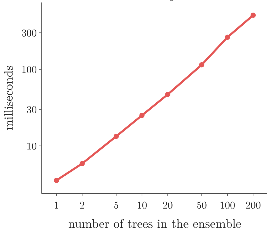
cost: training time
